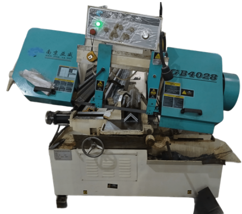
BANDSAW MACHINE
